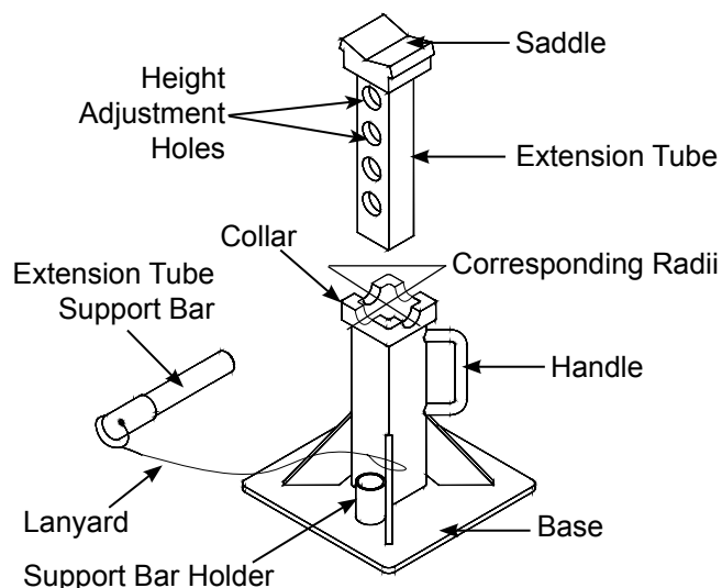
Figure 2 - Model 32225B Components
