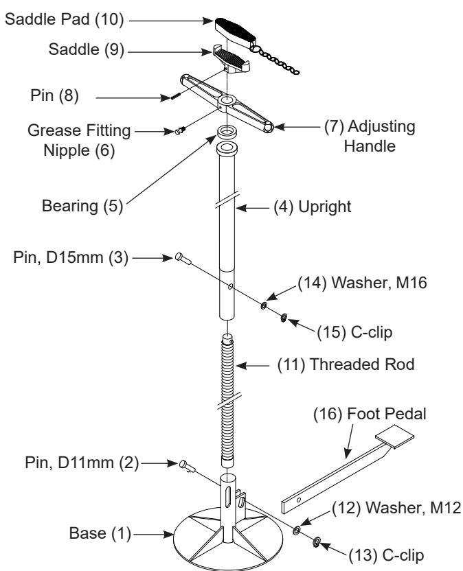
Figure 2 - BH5715 Nomenclature
