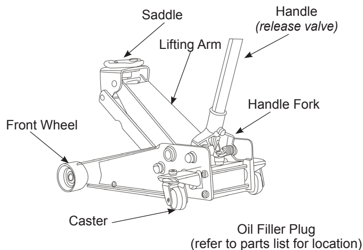
Figure 1 - Typical Jack Nomenclature
