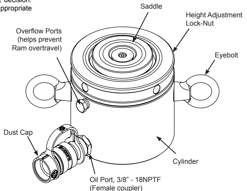
Figure 1 - Typical Lock-Nut Cylinder Components
