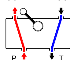
Position 1: Pressured oil flows to port A, port B returns flow to tank.
