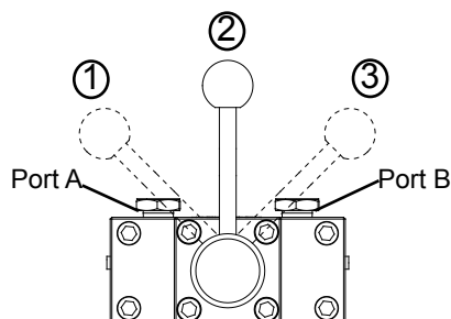
Figure 3 - Schematic flow path, valve position of 4-way, 3-position valve for Double Acting Cylinder
