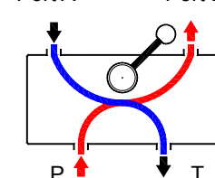
Position 3: Pressurized oil flows to port B, port A returns flow to tank.
