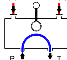
Position 2: Neutral, ports A & B are closed. Hold Position
