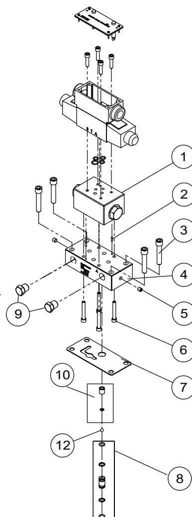
PS43L Parts Illustration
