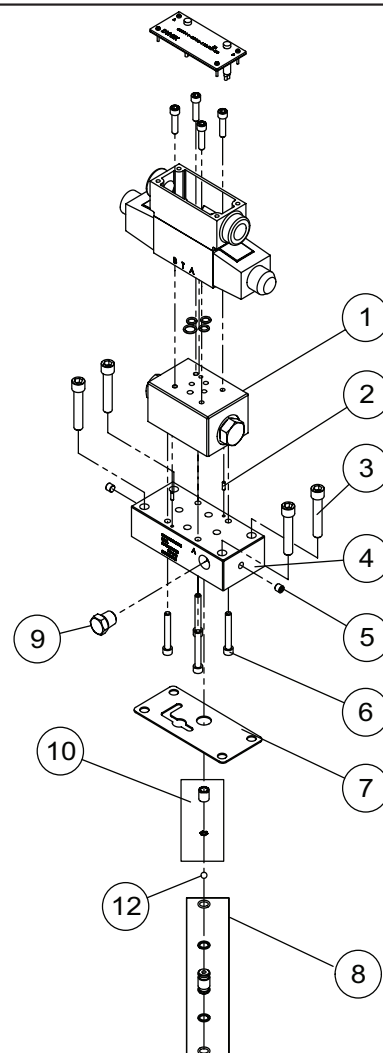
PS33L Parts Illustration
