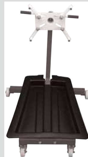
92510 : Oil Drip Pan Fits all Omega engine stands (Available separately)
